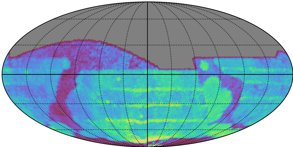
too_10_1v3.4_10yrs All sky all bands: Median Season Length
