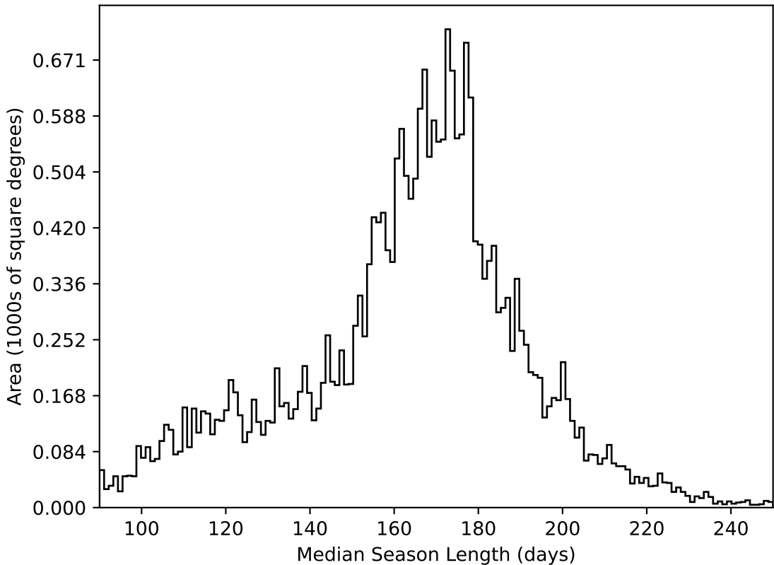
too_10_1v3.4_10yrs All sky all bands: Median Season Length
