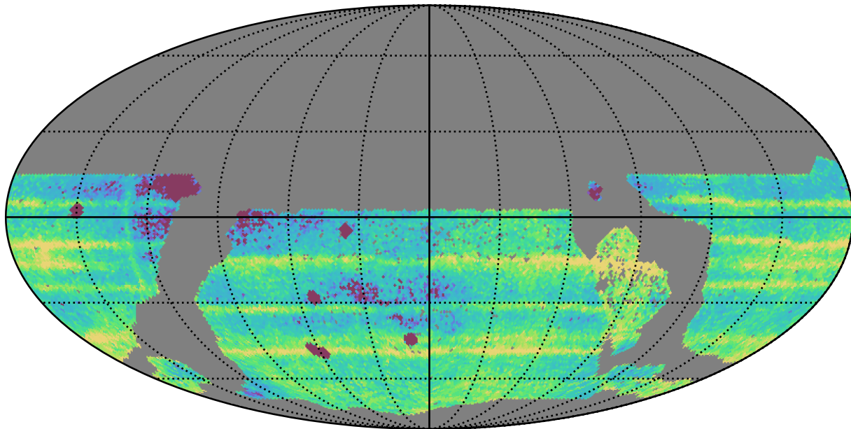
too_10_1v3.4_10yrs WFD: Median Intra-Night Gap
