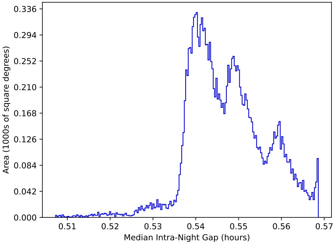
too_10_1v3.4_10yrs WFD: Median Intra-Night Gap
