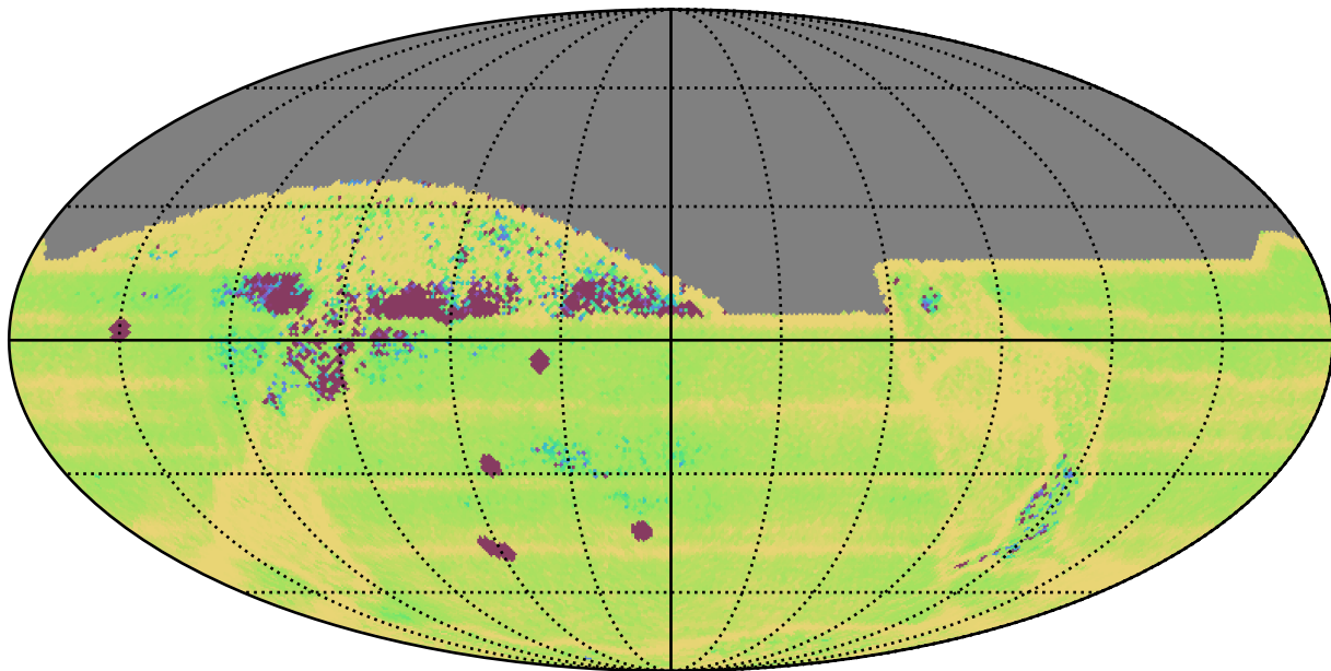
too_10_1v3.4_10yrs All sky: Median Intra-Night Gap
