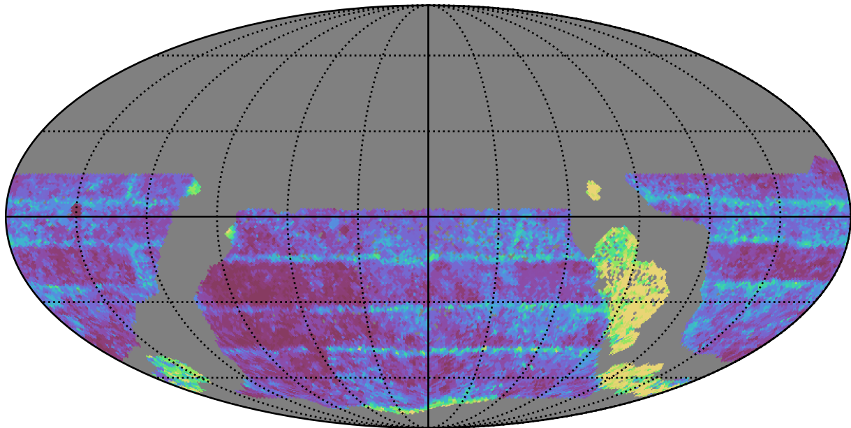
too_10_1v3.4_10yrs WFD z band: Median Inter-Night Gap
