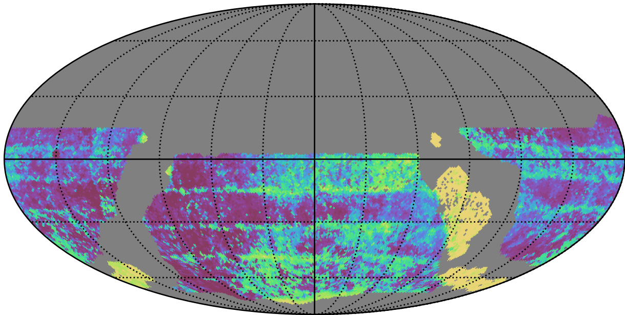
too_10_1v3.4_10yrs WFD y band: Median Inter-Night Gap
