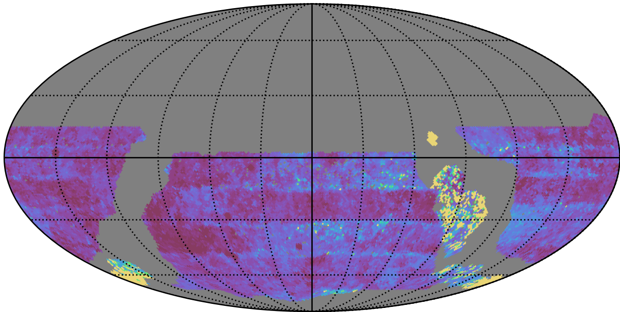
too_10_1v3.4_10yrs WFD u band: Median Inter-Night Gap
