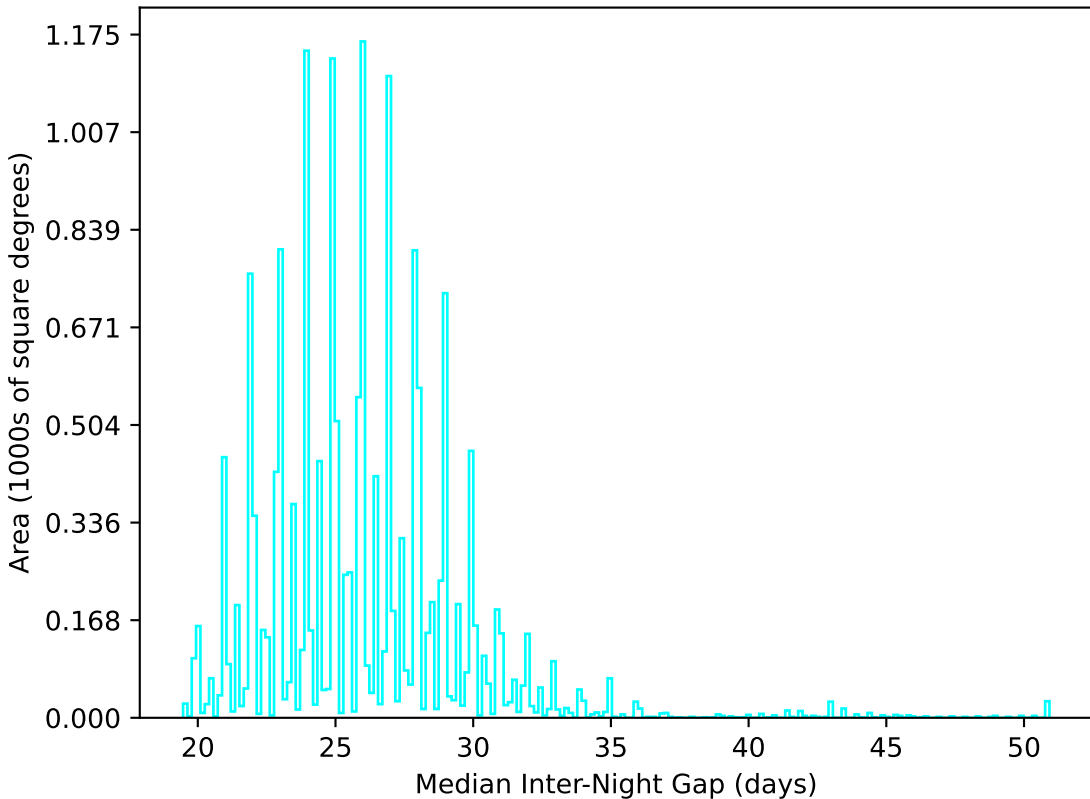
too_10_1v3.4_10yrs WFD u band: Median Inter-Night Gap
