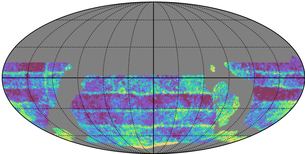
too_10_1v3.4_10yrs WFD r band: Median Inter-Night Gap
