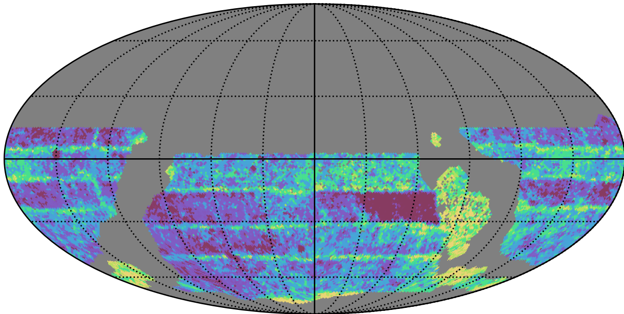
too_10_1v3.4_10yrs WFD i band: Median Inter-Night Gap
