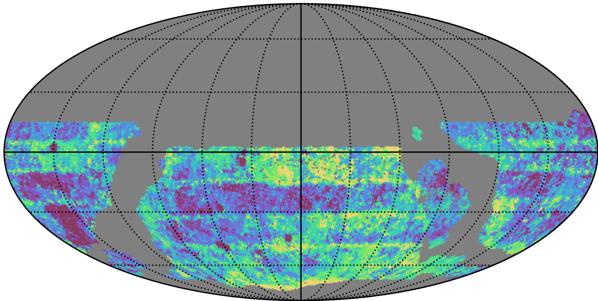
too_10_1v3.4_10yrs WFD g band: Median Inter-Night Gap
