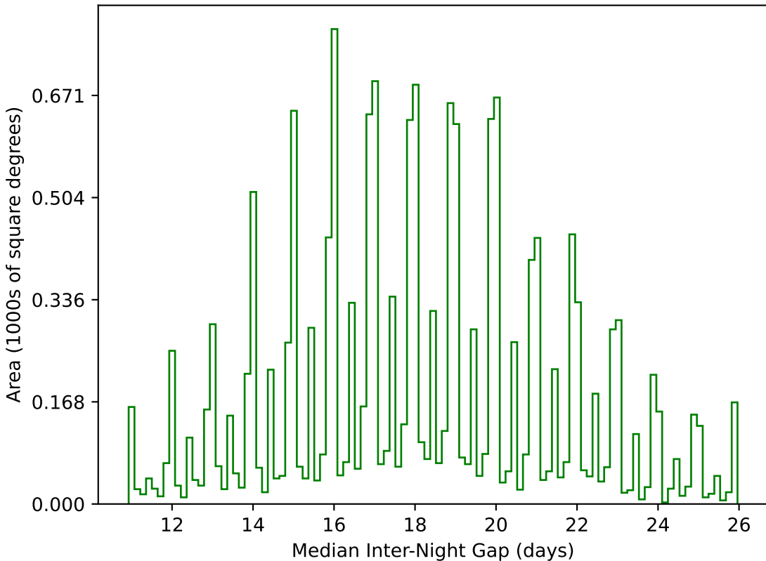
too_10_1v3.4_10yrs WFD g band: Median Inter-Night Gap
