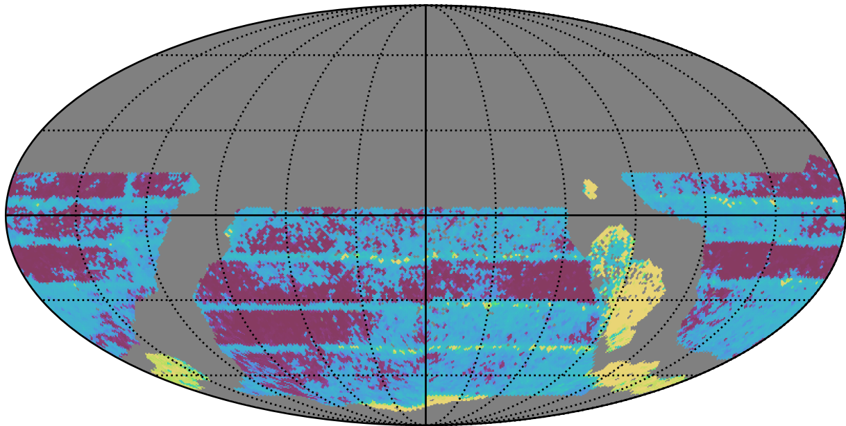
too_10_1v3.4_10yrs WFD all bands: Median Inter-Night Gap
