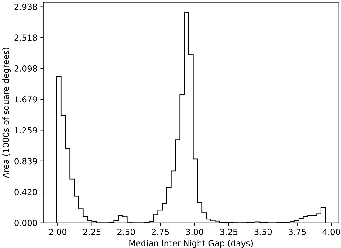
too_10_1v3.4_10yrs WFD all bands: Median Inter-Night Gap
