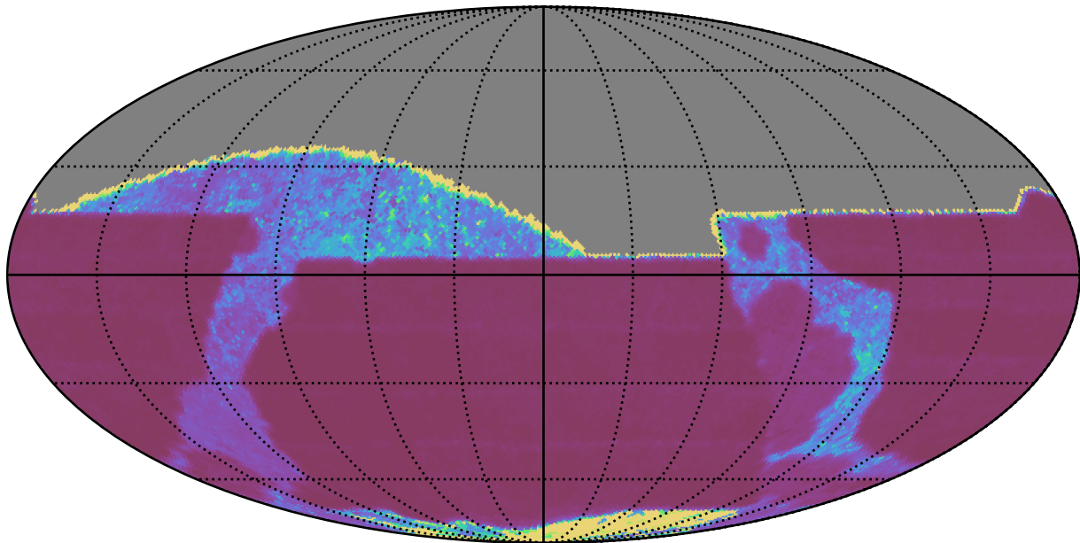
too_10_1v3.4_10yrs All sky z band: Median Inter-Night Gap
