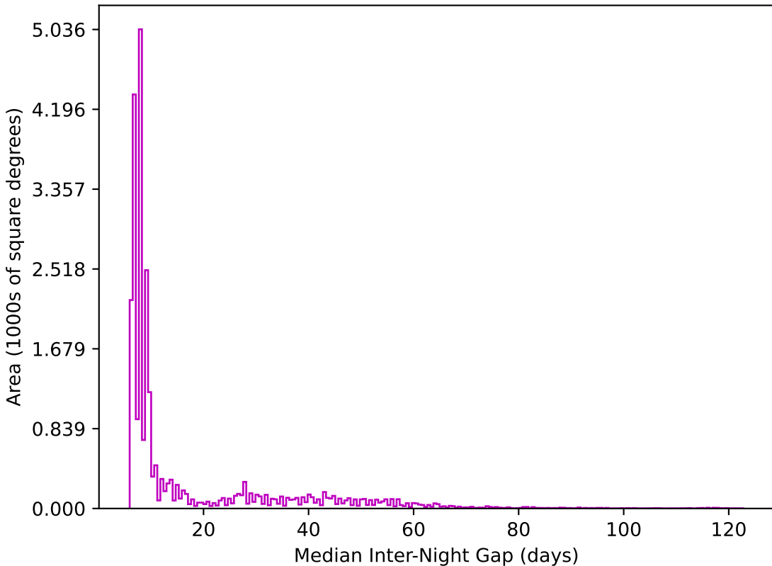
too_10_1v3.4_10yrs All sky z band: Median Inter-Night Gap
