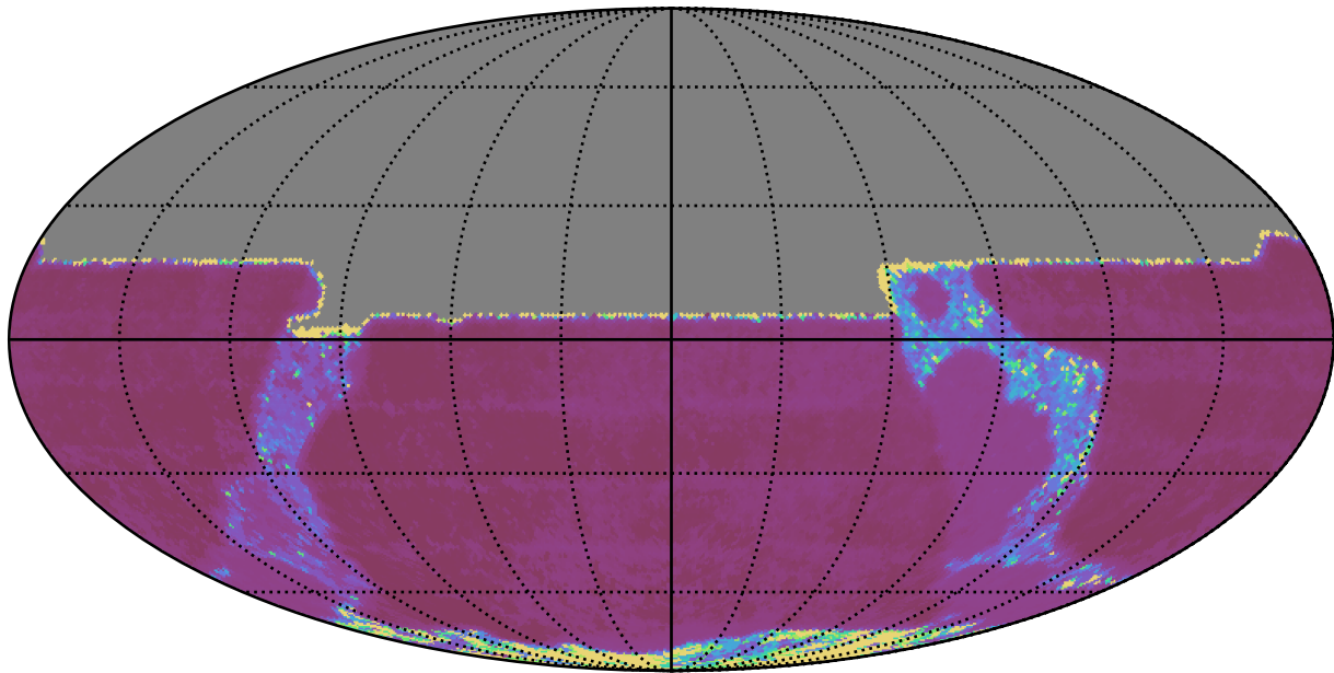
too_10_1v3.4_10yrs All sky y band: Median Inter-Night Gap
