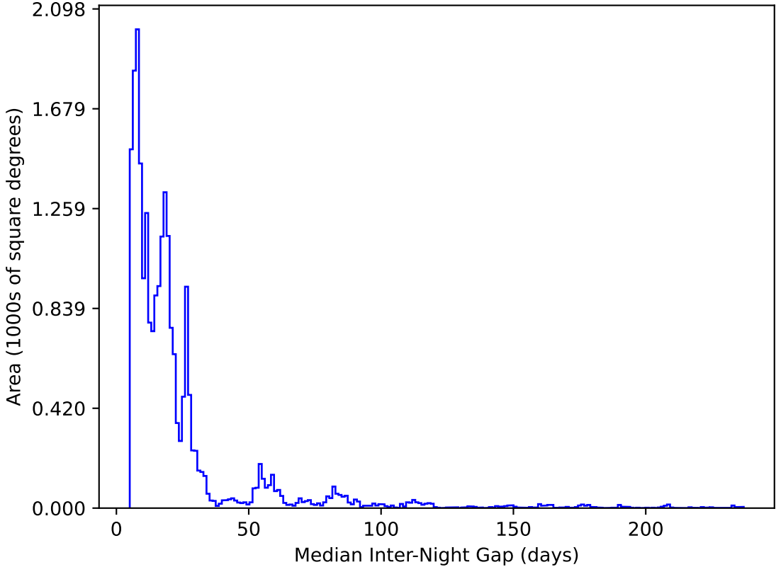
too_10_1v3.4_10yrs All sky y band: Median Inter-Night Gap
