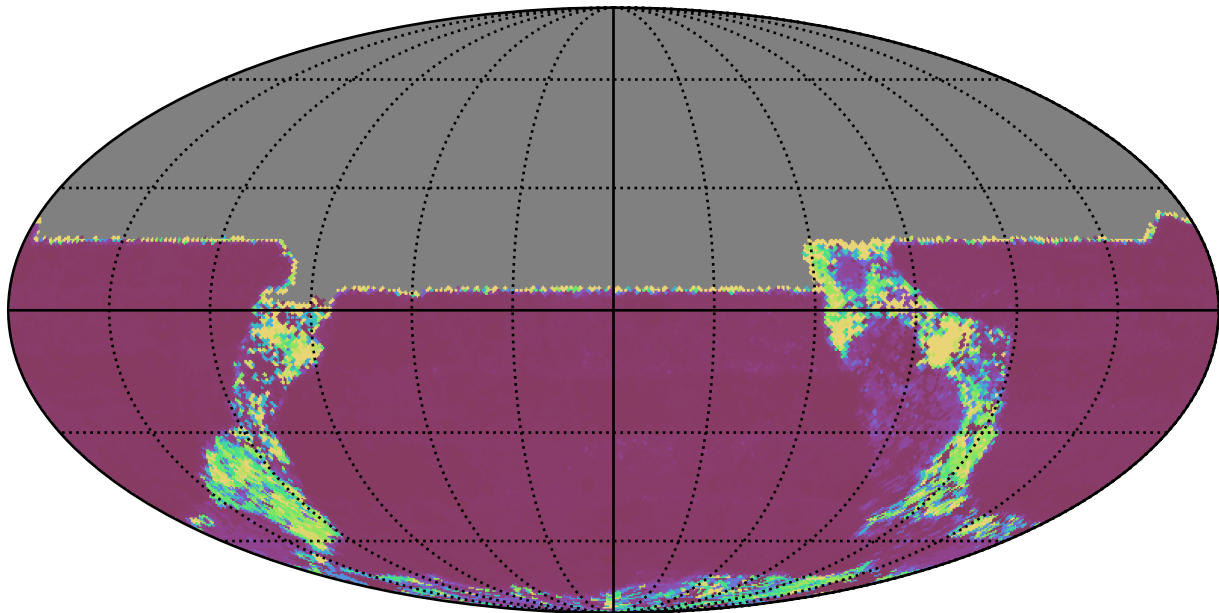
too_10_1v3.4_10yrs All sky u band: Median Inter-Night Gap
