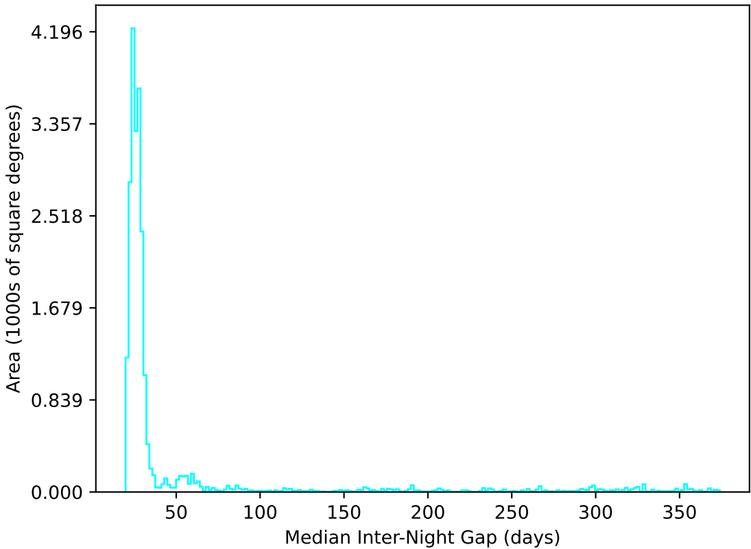
too_10_1v3.4_10yrs All sky u band: Median Inter-Night Gap
