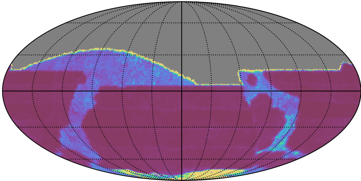
too_10_1v3.4_10yrs All sky r band: Median Inter-Night Gap
