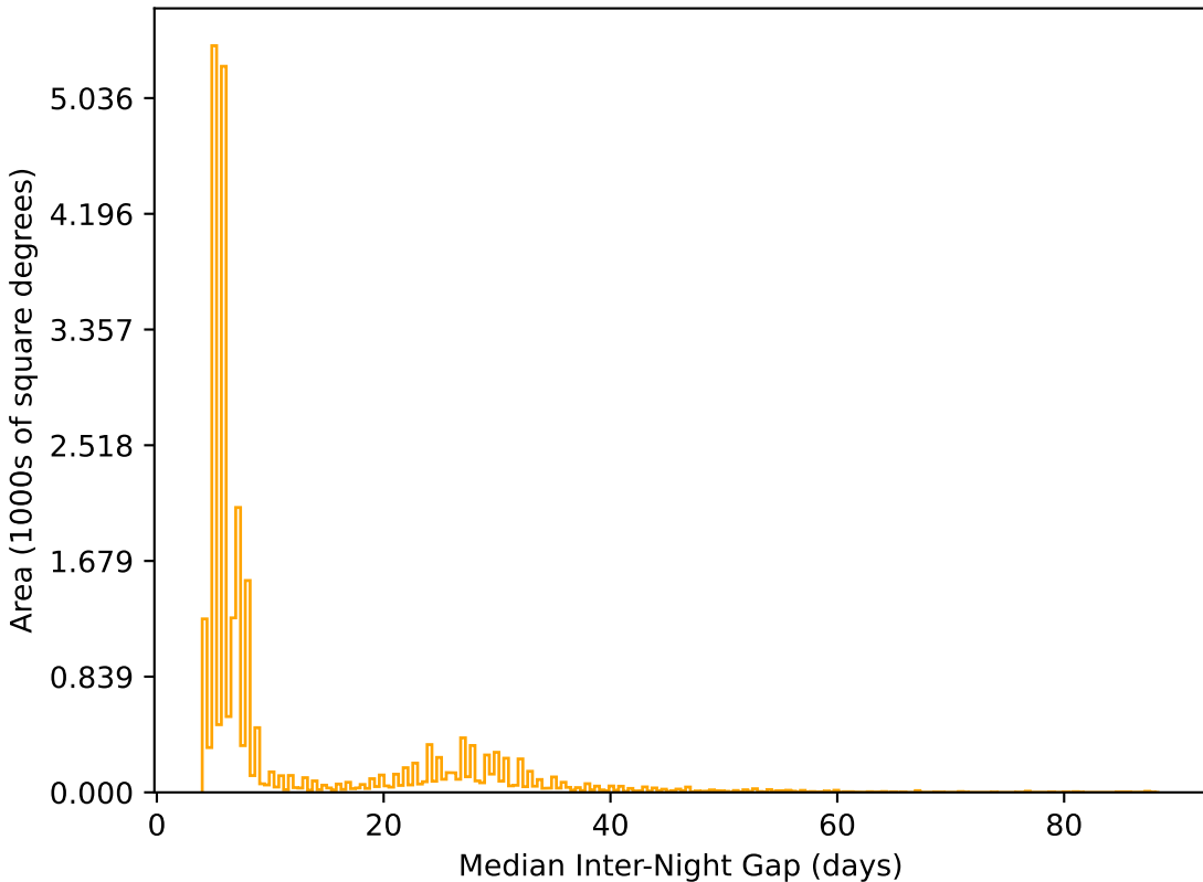
too_10_1v3.4_10yrs All sky r band: Median Inter-Night Gap
