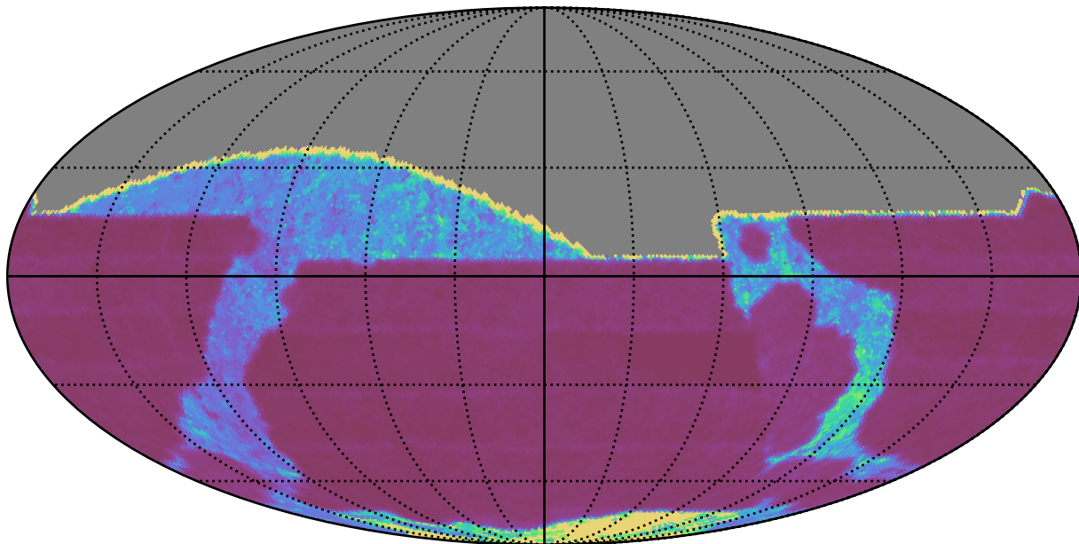
too_10_1v3.4_10yrs All sky i band: Median Inter-Night Gap
