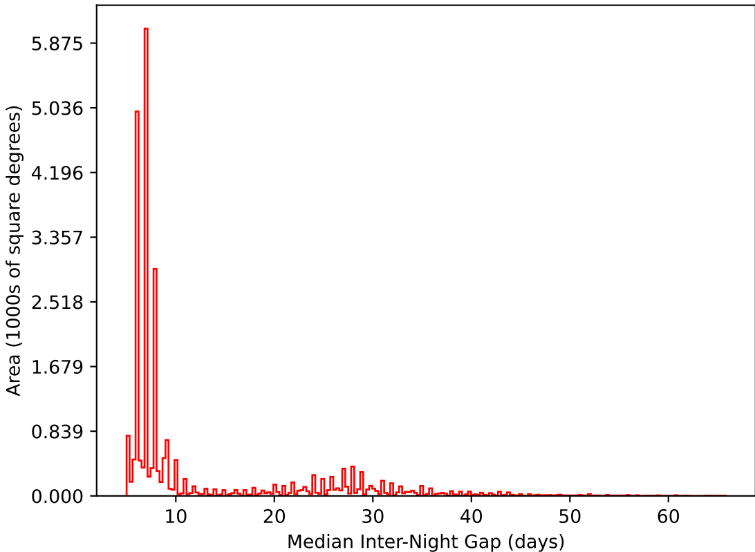
too_10_1v3.4_10yrs All sky i band: Median Inter-Night Gap
