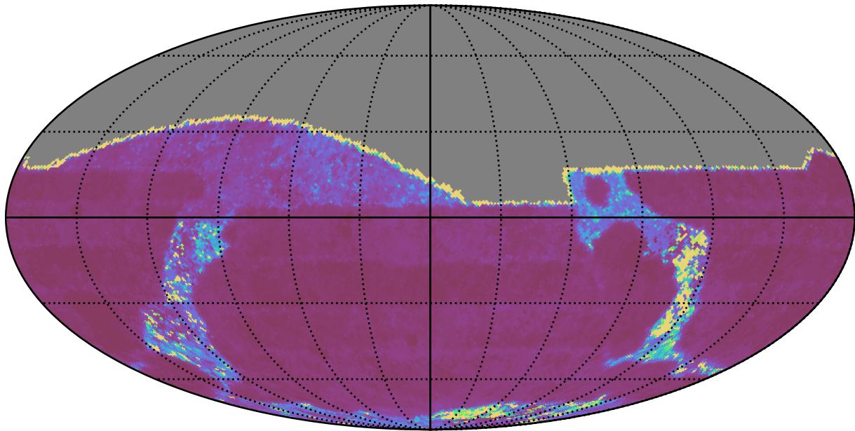
too_10_1v3.4_10yrs All sky g band: Median Inter-Night Gap
