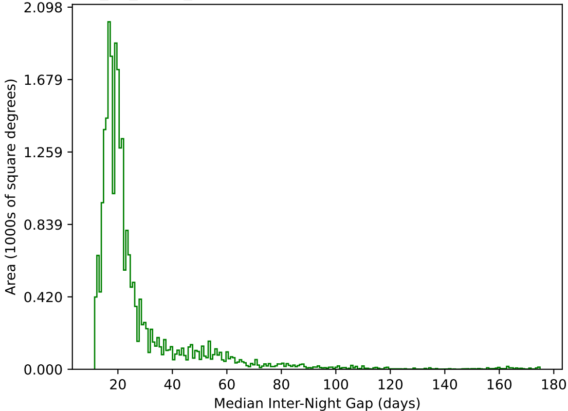
too_10_1v3.4_10yrs All sky g band: Median Inter-Night Gap
