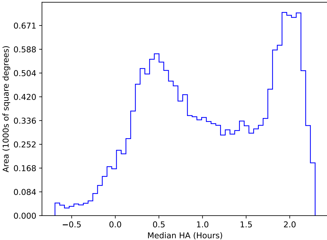
too_10_1v3.4_10yrs WFD z band: Median HA
