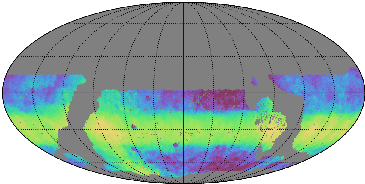
too_10_1v3.4_10yrs WFD y band: Median HA
