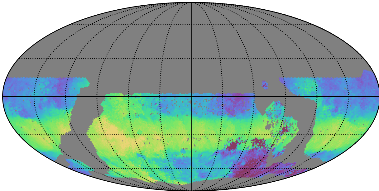
too_10_1v3.4_10yrs WFD u band: Median HA
