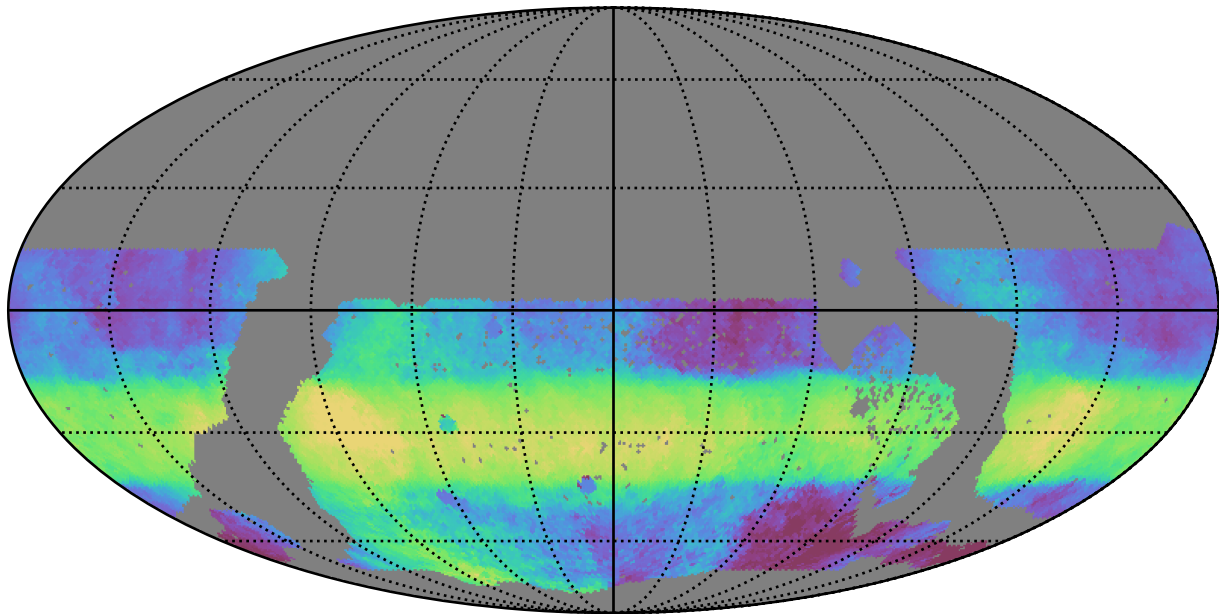
too_10_1v3.4_10yrs WFD r band: Median HA
