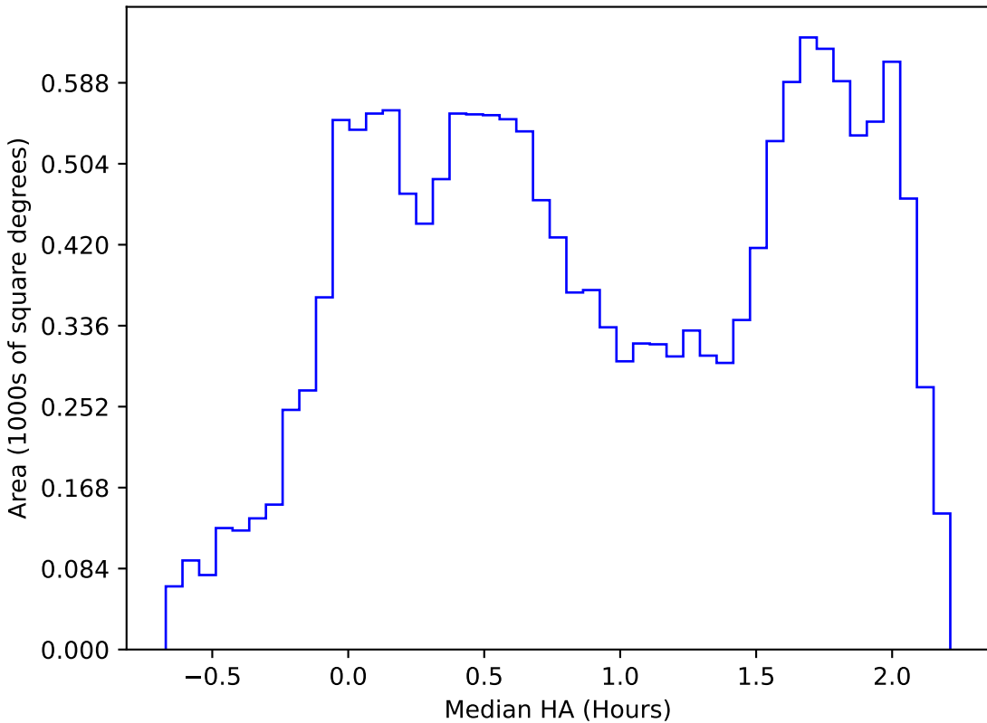
too_10_1v3.4_10yrs WFD r band: Median HA
