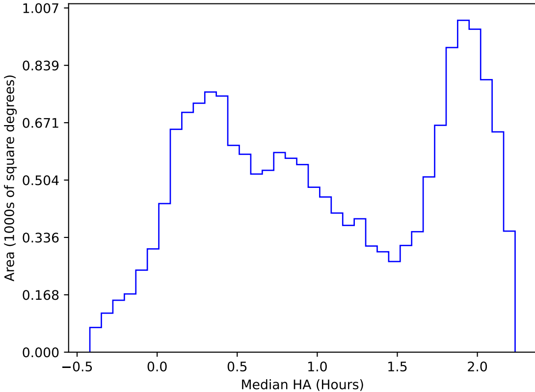
too_10_1v3.4_10yrs WFD i band: Median HA
