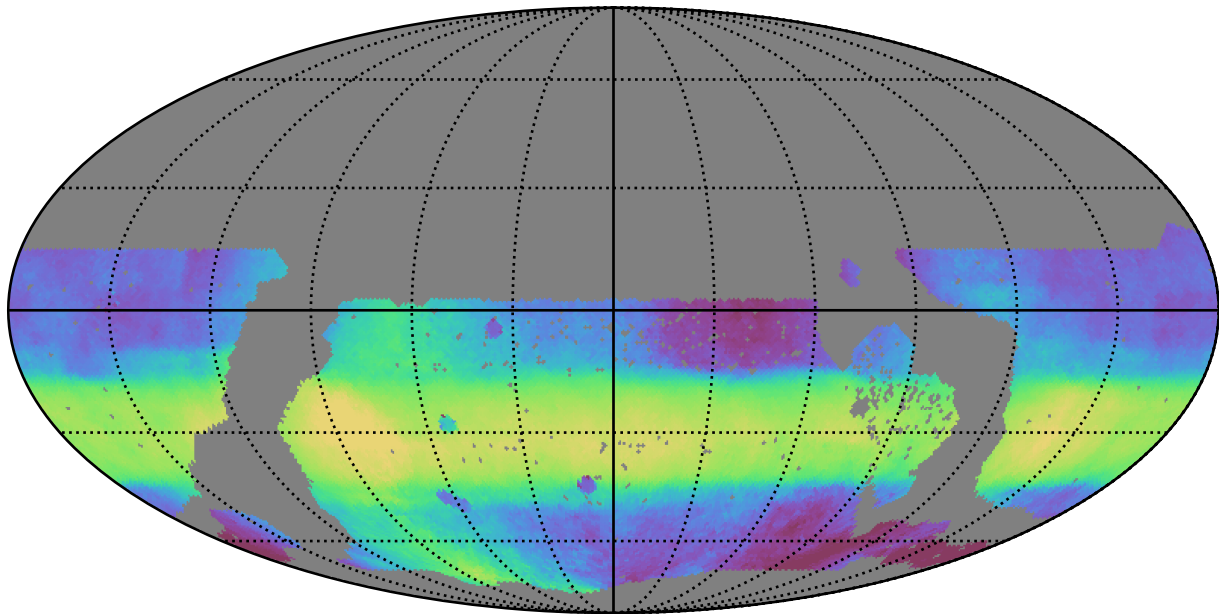
too_10_1v3.4_10yrs WFD all bands: Median HA
