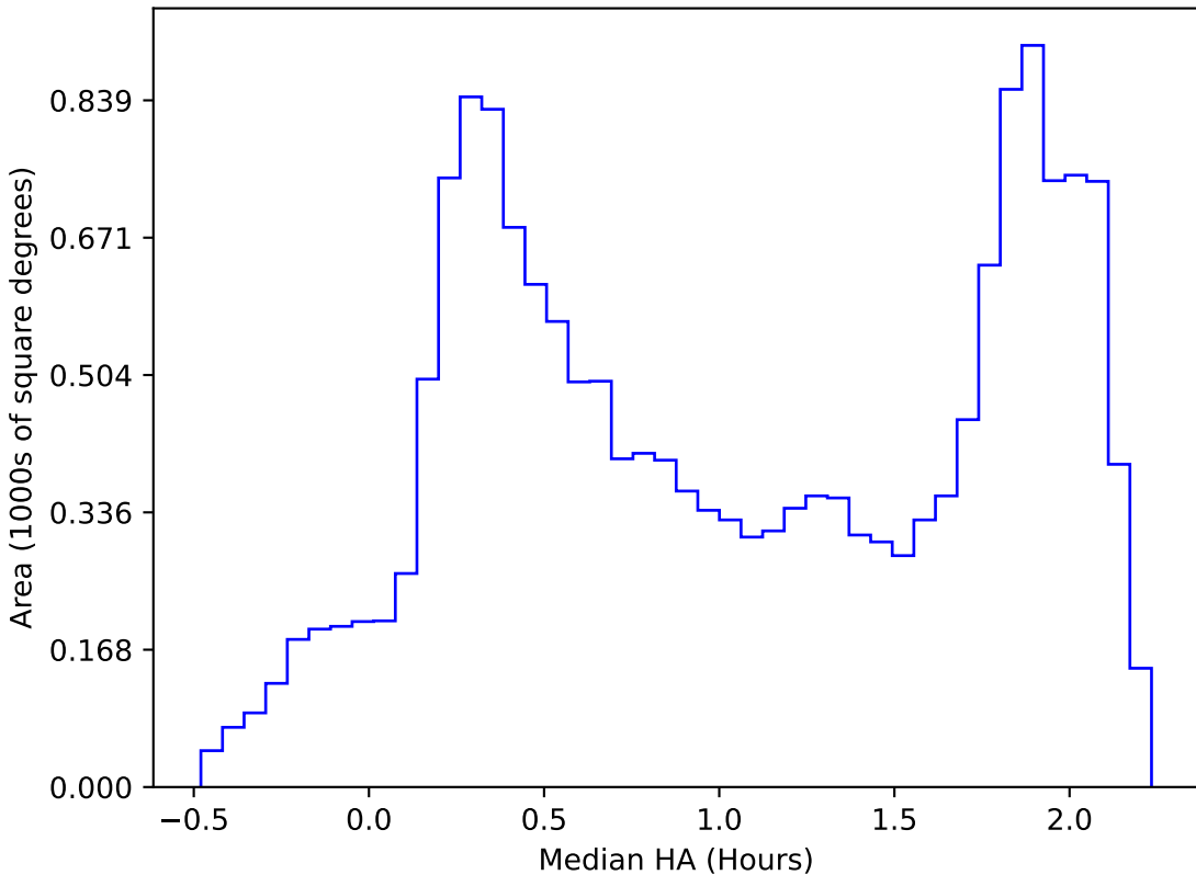
too_10_1v3.4_10yrs WFD all bands: Median HA
