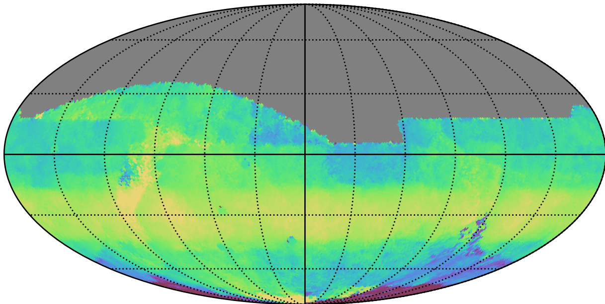
too_10_1v3.4_10yrs All sky z band: Median HA
