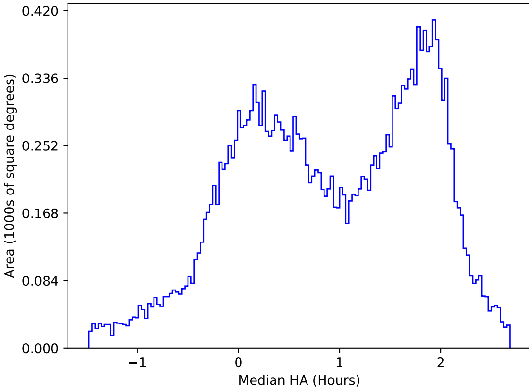
too_10_1v3.4_10yrs All sky u band: Median HA
