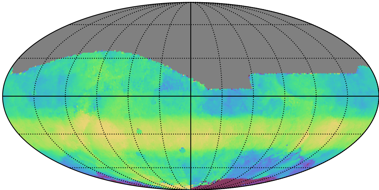
too_10_1v3.4_10yrs All sky r band: Median HA
