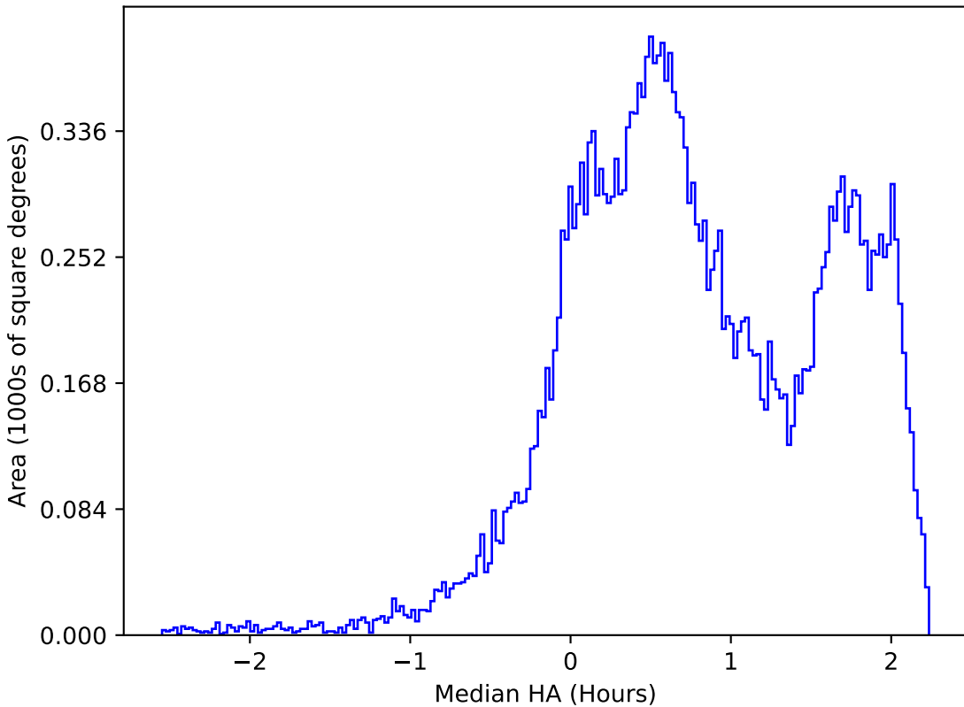
too_10_1v3.4_10yrs All sky r band: Median HA
