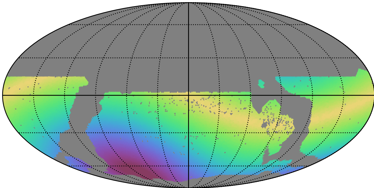
too_10_1v3.4_10yrs WFD z band: Max solarElong
