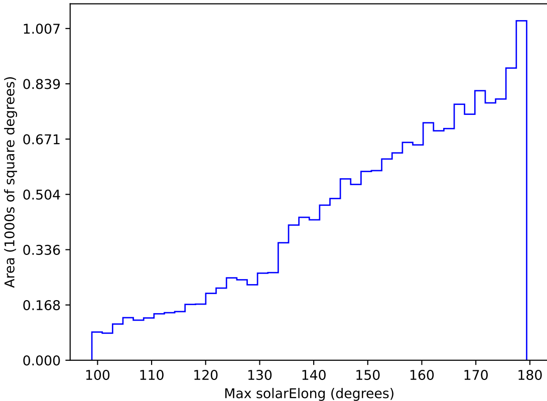
too_10_1v3.4_10yrs WFD z band: Max solarElong
