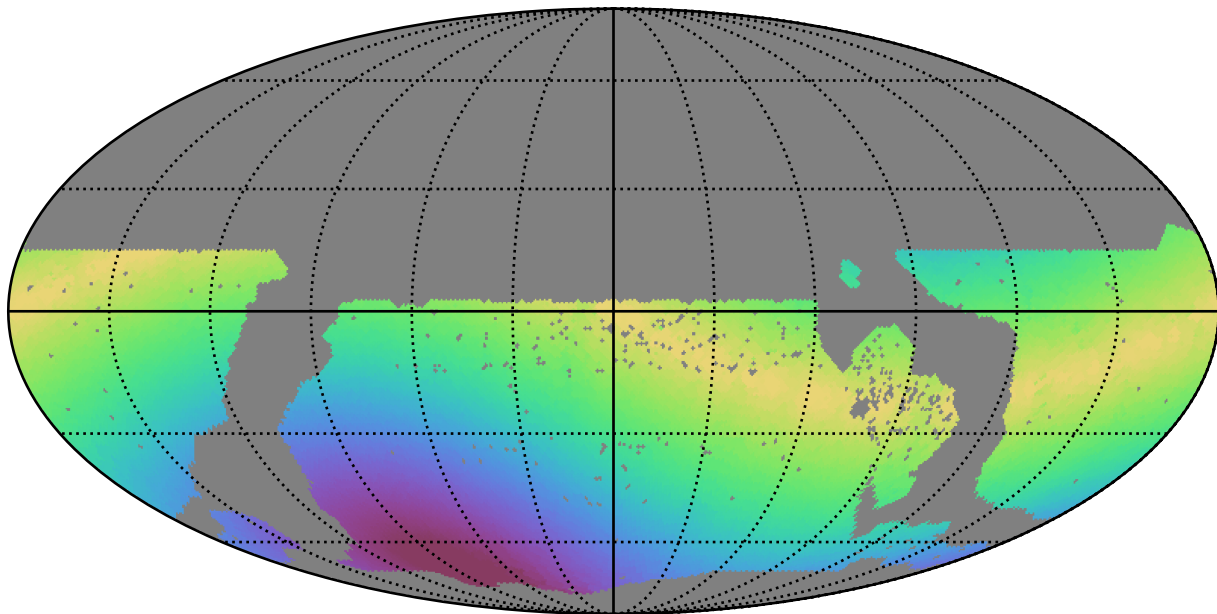
too_10_1v3.4_10yrs WFD u band: Max solarElong
