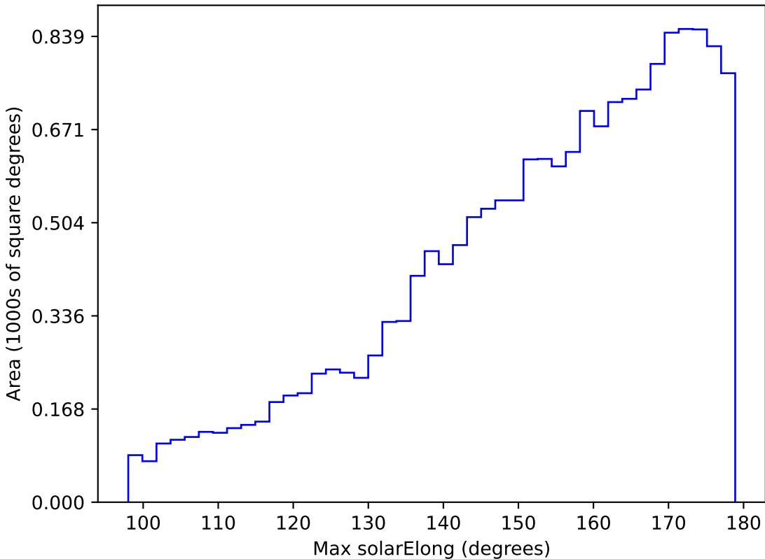
too_10_1v3.4_10yrs WFD u band: Max solarElong
