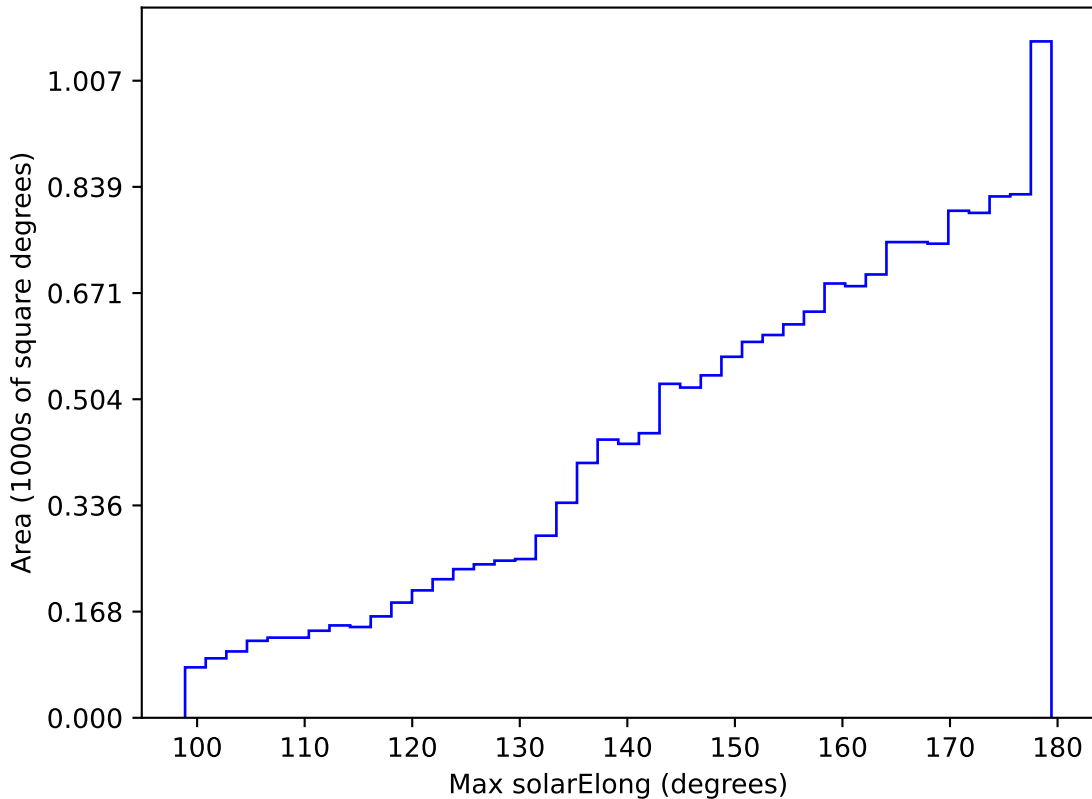
too_10_1v3.4_10yrs WFD r band: Max solarElong
