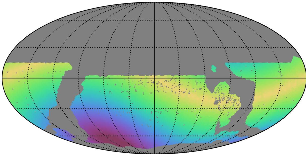
too_10_1v3.4_10yrs WFD g band: Max solarElong
