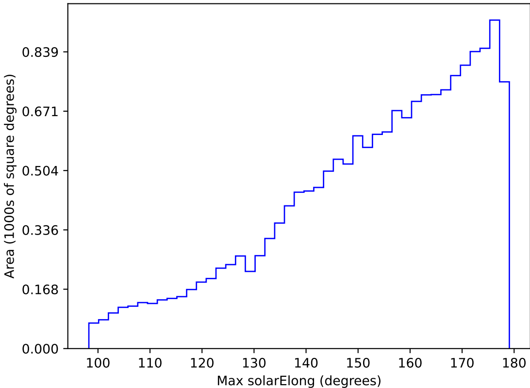
too_10_1v3.4_10yrs WFD g band: Max solarElong
