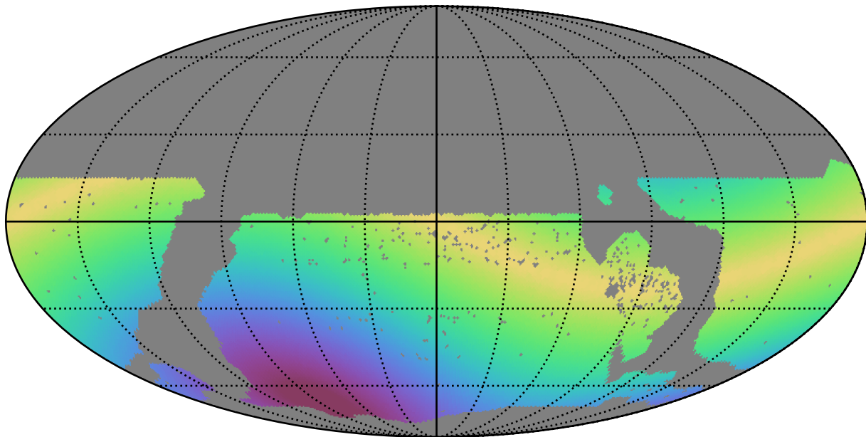
too_10_1v3.4_10yrs WFD all bands: Max solarElong
