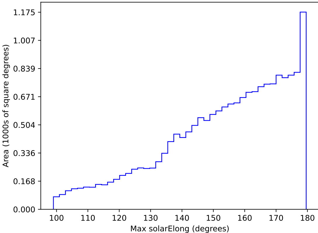
too_10_1v3.4_10yrs WFD all bands: Max solarElong
