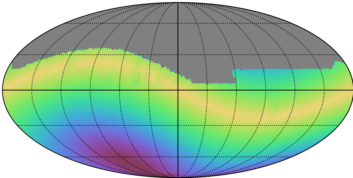
too_10_1v3.4_10yrs All sky z band: Max solarElong
