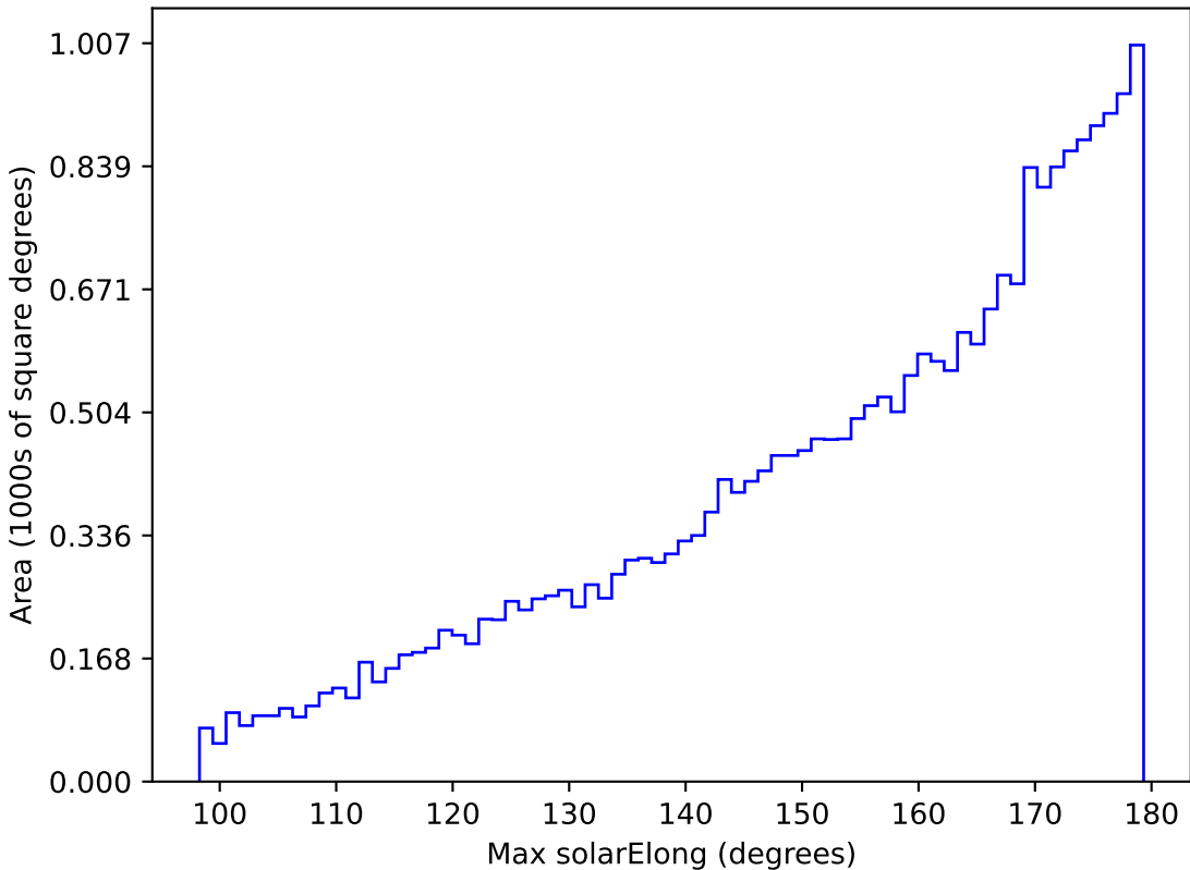
too_10_1v3.4_10yrs All sky z band: Max solarElong
